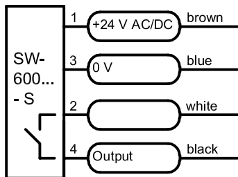
Connection fig. 3
